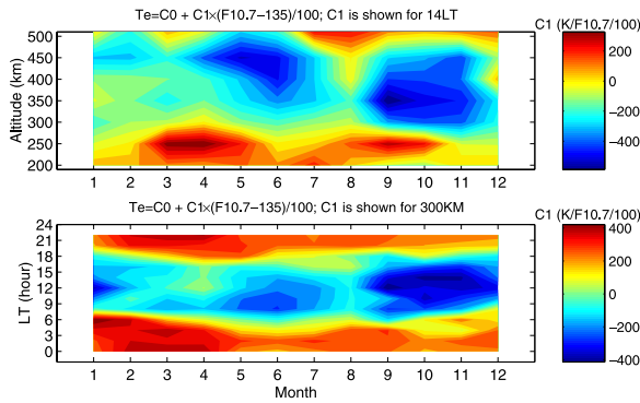
Figure 7. Te dependences on the solar activity at different heights, local times, and months. Coefficient C_1 in Te = C_0 + C_1 \times f is shown, where f = (F10.7 - 135)/100 is the normalized F10.7 and C_0 is the background Te independent of solar activity. C_1 represents the slope of the Te change with respect to f change. C_0 and C_1 are obtained by the least-squares fit using the paired Te and f data. C_1 is shown here in the unit of ^{\circ}\text{K} per 100 F10.7 units.
