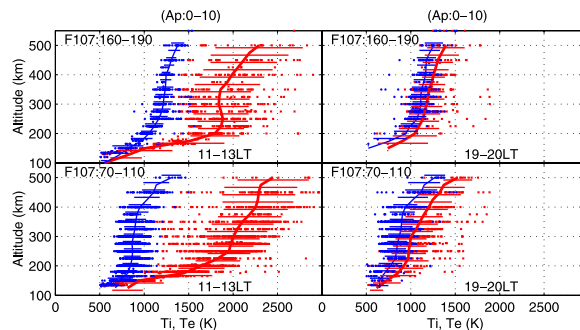
Figure 6. Ti and Te altitude profiles at two local time spans for two solar activity levels. The blue circles are for Ti and the red dots are for Te.
