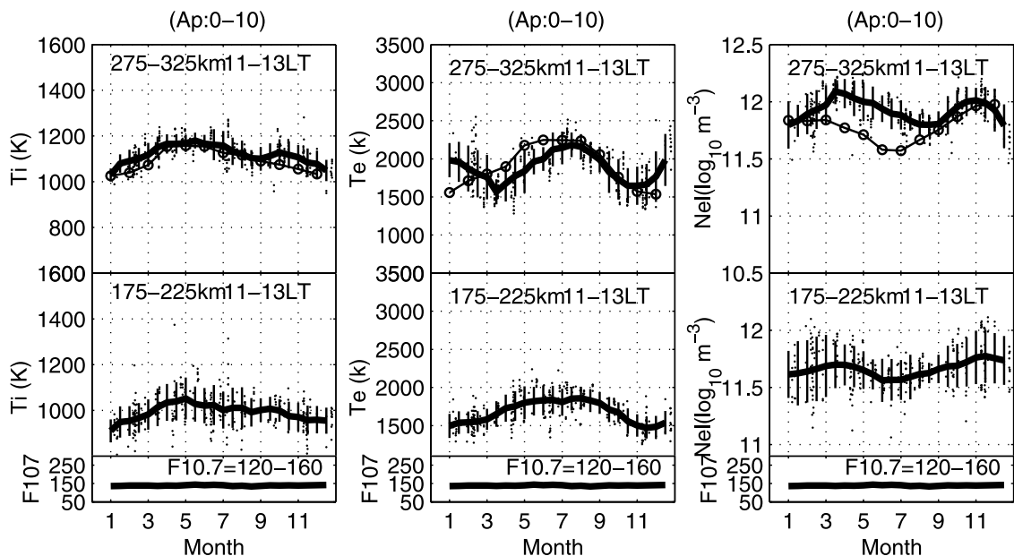
Figure 3. Seasonal variations of the midday T_i , T_e , and N_e at two altitude ranges for F10.7 between 120 and 160 units. Millstone Hill empirical model values are represented by the line and circle curve for 300 km at 1200 LT with F10.7 = 140 units.
